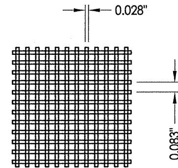
16 WIRE CLOTH MESH (12 X12) Wire diameter: 0.028" Stainless Steel (304) open area: 56%
