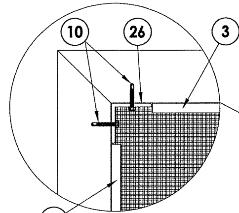
SCREEN CORNER DETAIL Lock side only
