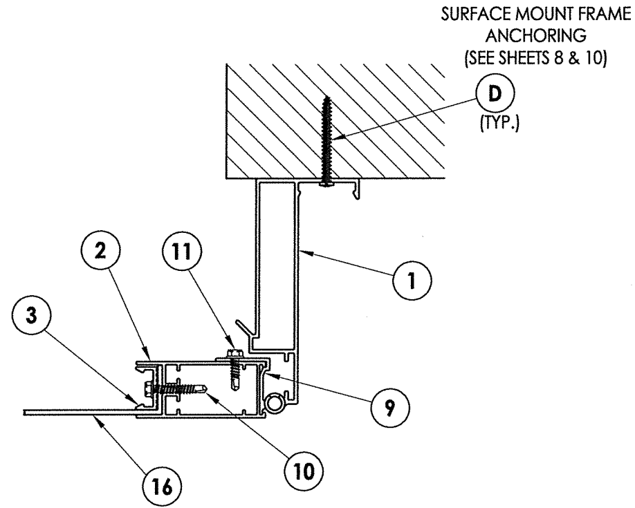
2 4 HORIZONTAL CROSS SECTION
