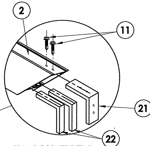
FRAME CORNER DETAIL
