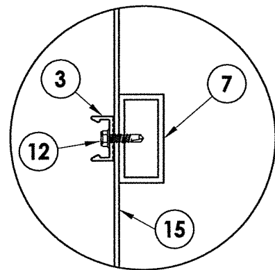
HORIZONTAL SUPPORT BAR DETAIL Horizontal bar required at centerline for all panel heights > 48" and at 1/3 points for all panel heights > 96"
